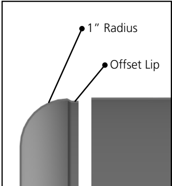
Offset tub-cap lip seats underneath edge of tub skin, creating an easy to align overlap joint with flush outer surface.
